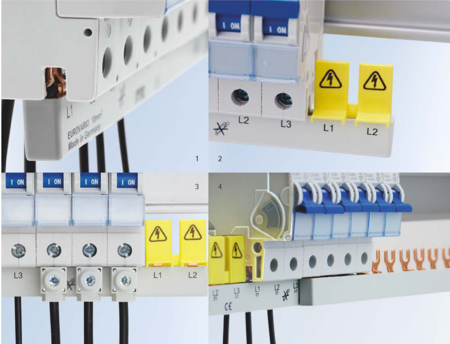
picture 1: integrated endcover | picture 2: protection covers for unused lugs | picture 3: application with connection terminal | picture 4: Interconnection of several eurovario busbars
